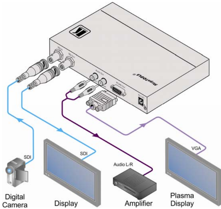
Figure 2: Connecting the VP-473 3G HD-SDI to PC/HD Scaler
