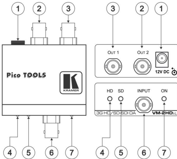
Figure 1: VM-2HDxL 3G HD/SD – SDI DA
